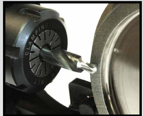
Step Drills
