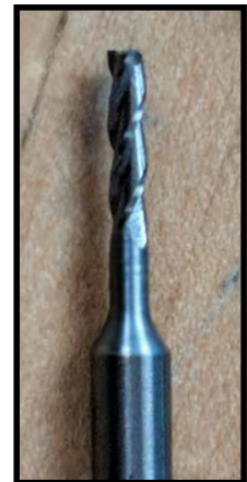
Chamfer on one side to reinforce neck reduction
